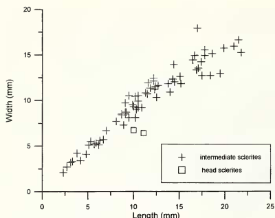
TEXT-FIG. 5. Length-width graph for intermediate and head sclerites of Chelodes actinis sp. nov.
